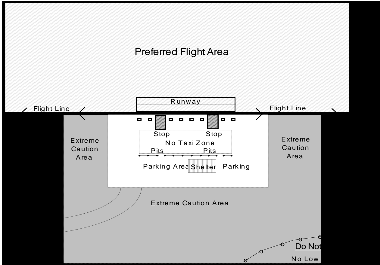
Figure 1 Flying Field Layout.
